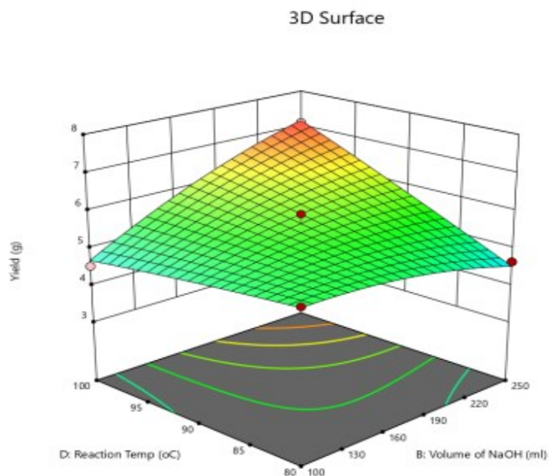
Figure 10: Response surface 3D plot for the interaction between volume of NaOH and reaction temperature
