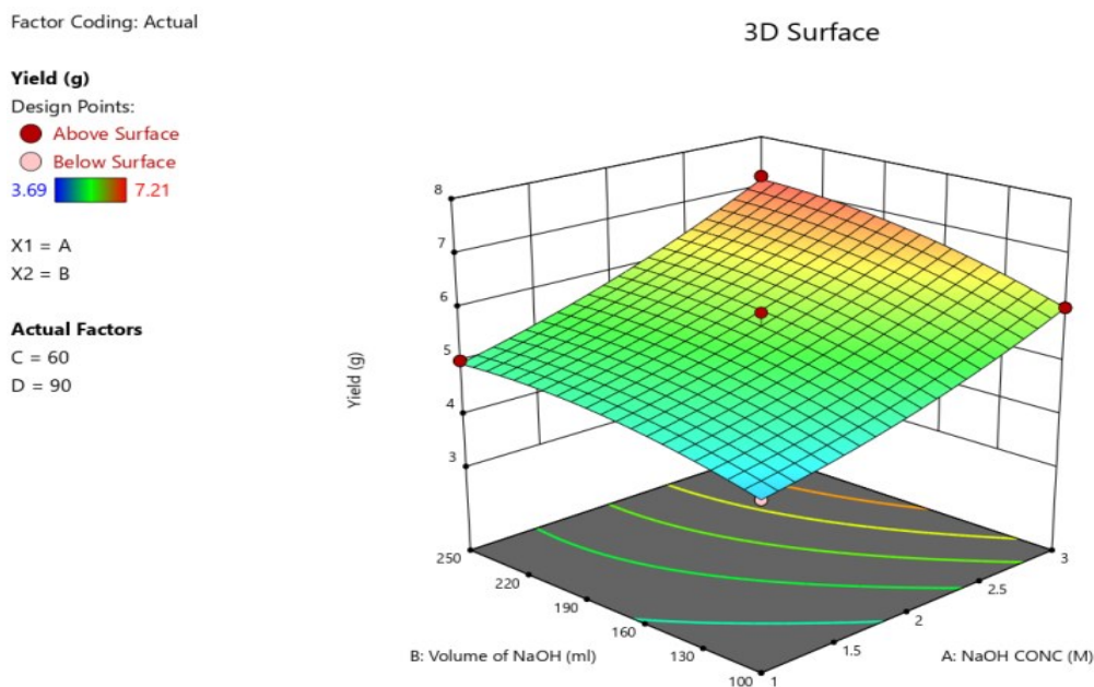
Figure 6: Response surface plot for the interaction between the volume and NaOH concentrations
