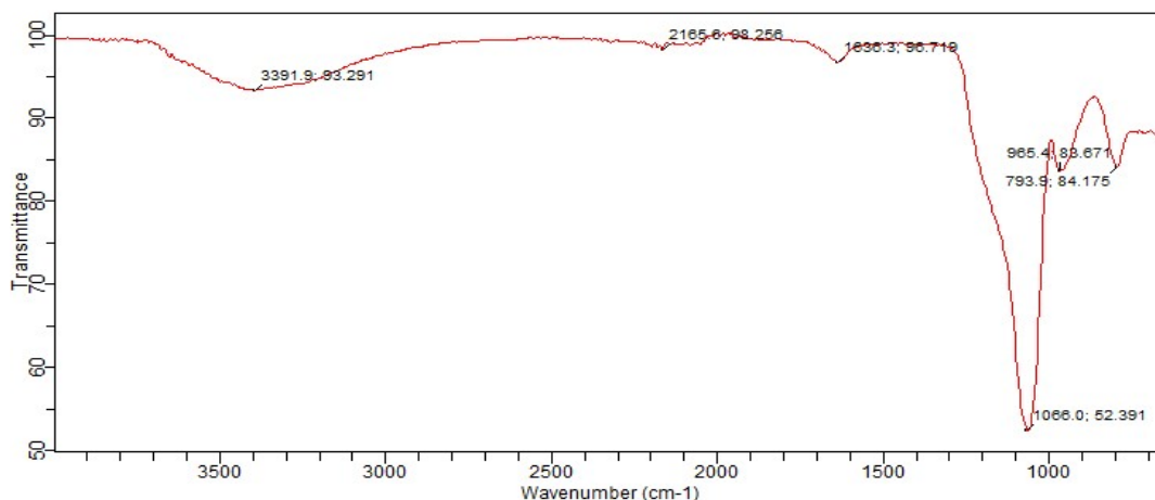
Figure 13: FTIR Spectrum Amorphous Silica
