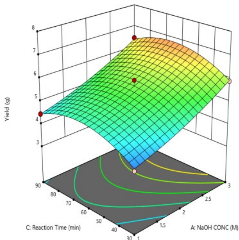
Figure 7: Response surface 3D plot for the interaction between reaction time and NaOH concentration
