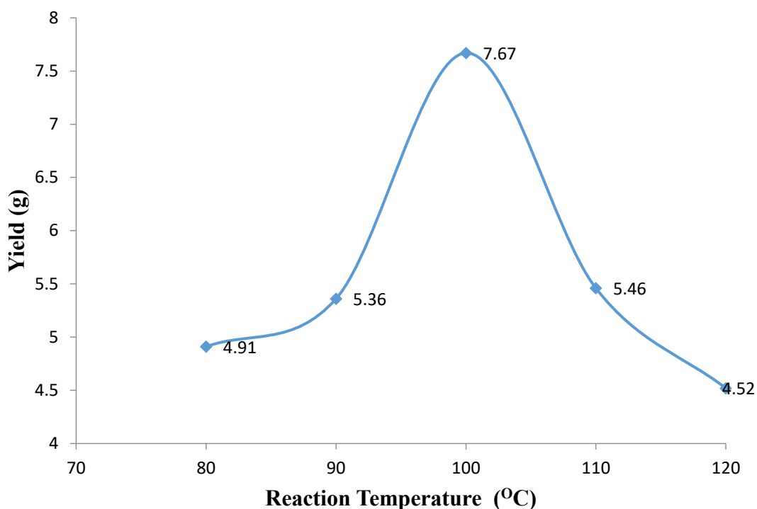
Figure 4: Effects of reaction temperature on the yield of silica from 10 g of rice husk ash
