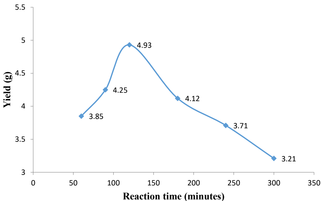
Figure 3: Effects of reaction time on the yield of silica from 10 g of rice husk ash
