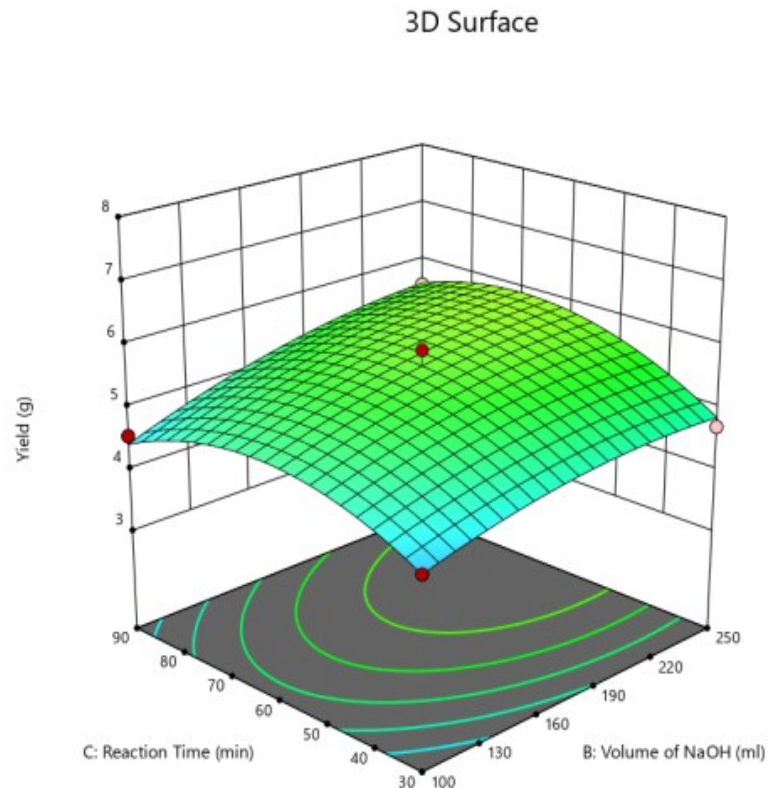
Figure 9: Response surface 3D plot for the interaction between reaction time and volume of NaOH
