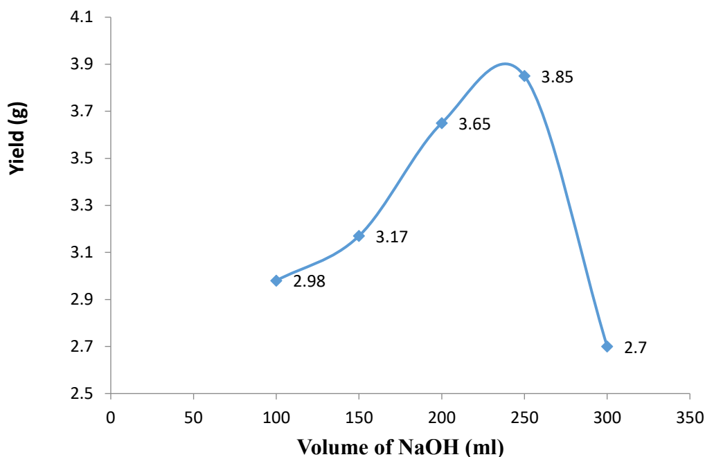
Figure 2: Effects of volume of NaOH on the yield of silica from 10 g of rice husk ash
