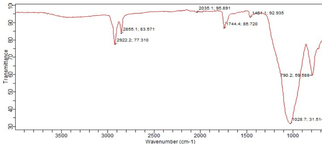
Figure 12: FT-IR Spectrum of rice husk ash
