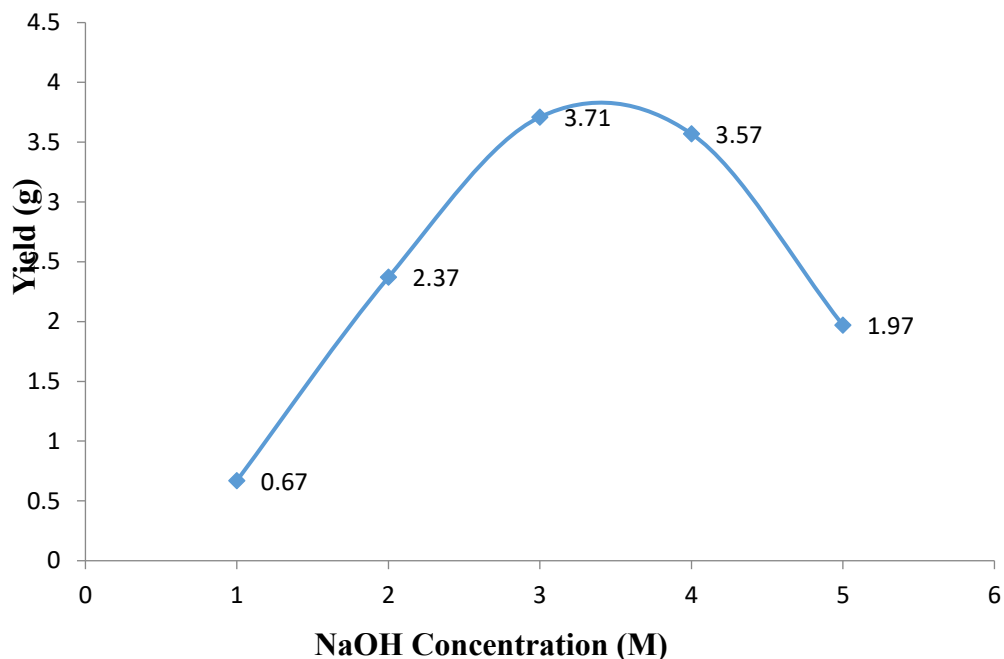
Figure 1: Effects of NaOH concentration on the yield of silica from 10 g of rice husk ash
