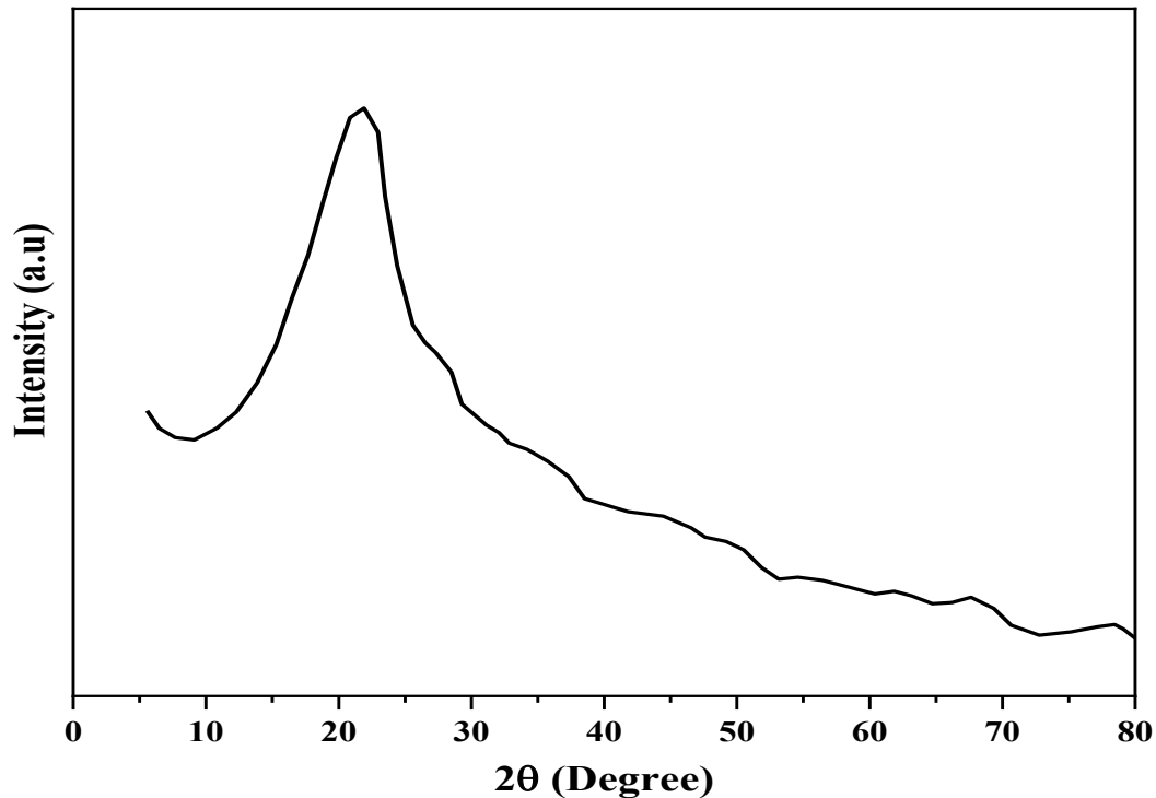
Figure 15: XRD analysis of amorphous silica
