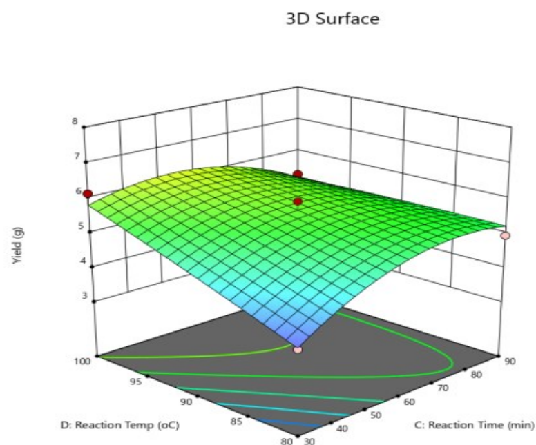
Figure 11: Response surface 3D plot for the interaction between reaction time and reaction temperature
