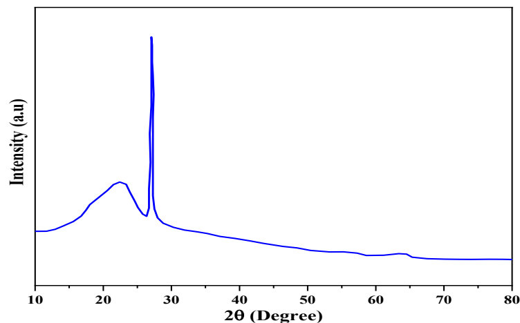
Figure 14: XRD pattern of rich husk ash produced at 700 °C
